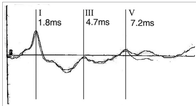
Figure 3. Notice the large increase in the I-V inter-peak interval and the low wave V amplitude.
